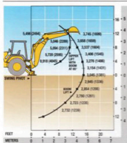
310SE BACKHOE WITH STANDARD DIPPERSTICK
