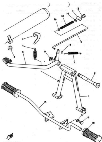
FIG. 24 STAND, REST
