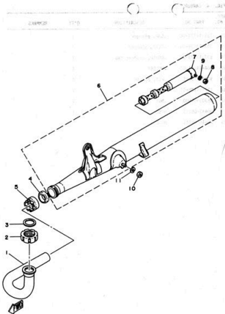
FIG. 5 EXHAUST
