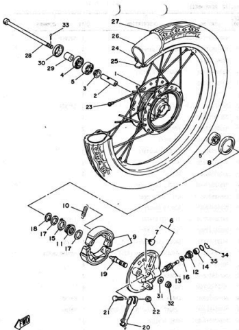
FIG. 21 FRONT VIEW
